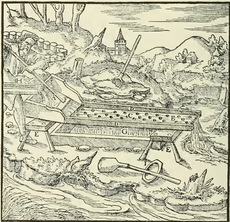
A—HEAD OF FRAME. B—FRAME. C—HOLES. D—EDGE-BOARDS. E—STOOLS F—SCRUBBER. G—TROUGH. H—LAUNDER. I—BOWL.
